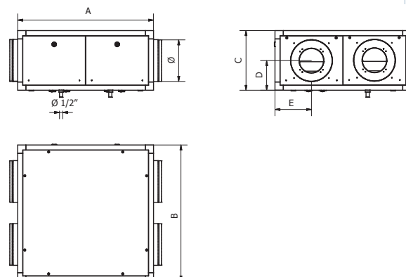
DIMENSIONS (mm) and WEIGHT (Kg) WITHOUT BY-PASS
